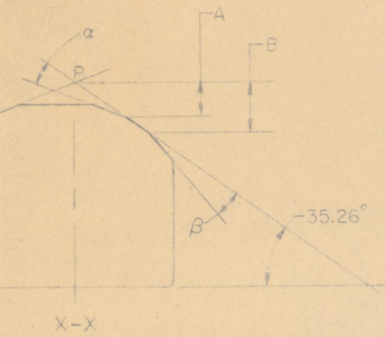
SHOULDER MODIFICATIONS
