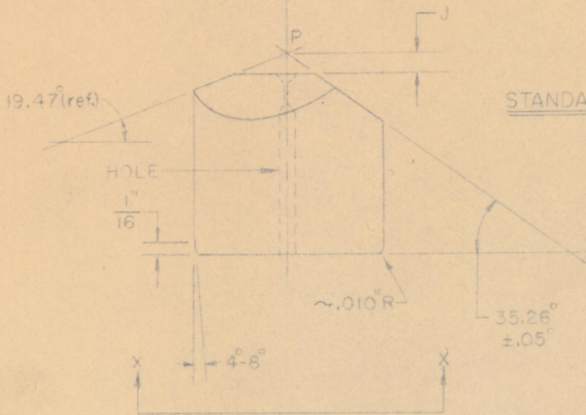
STANDARD ANVIL
